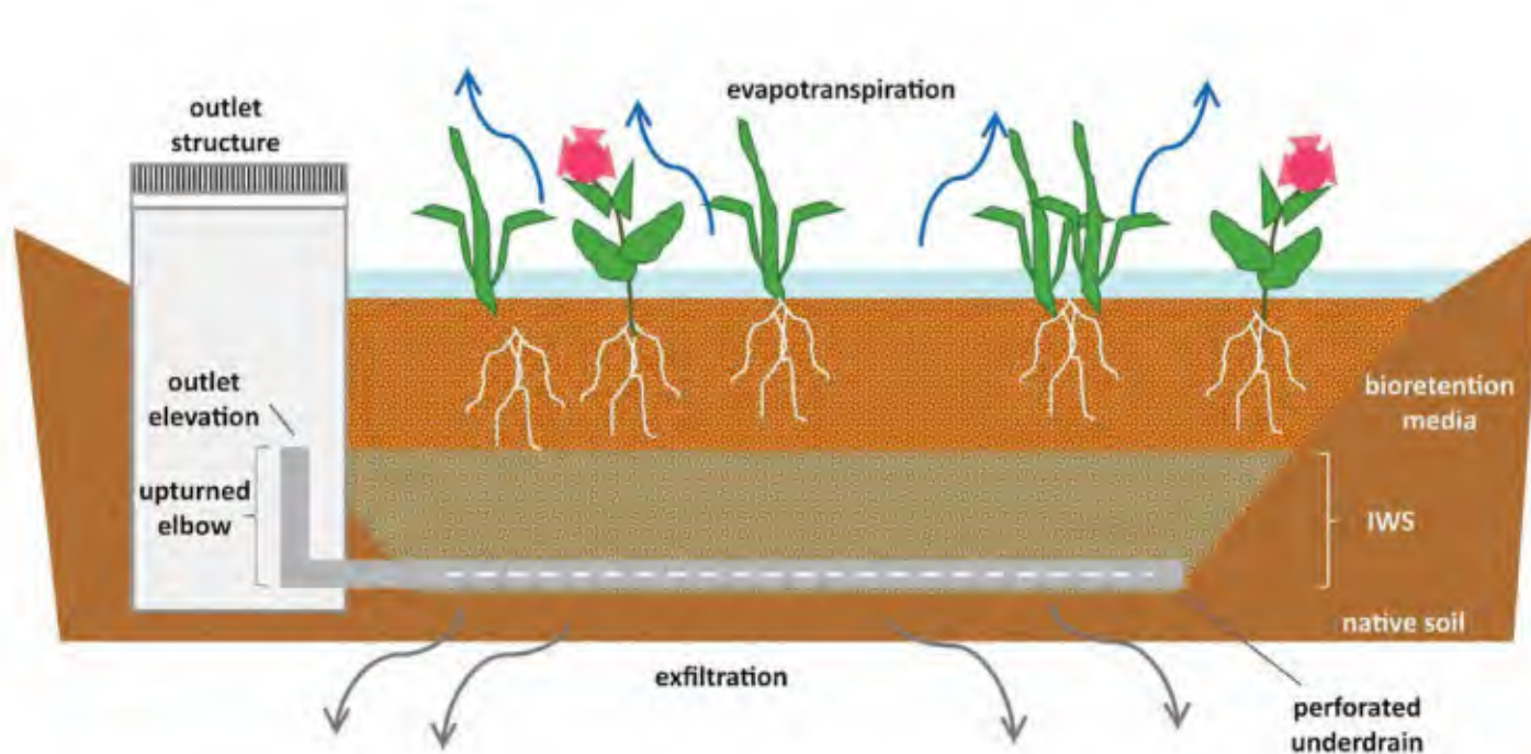
Conceptual IWS schematic
