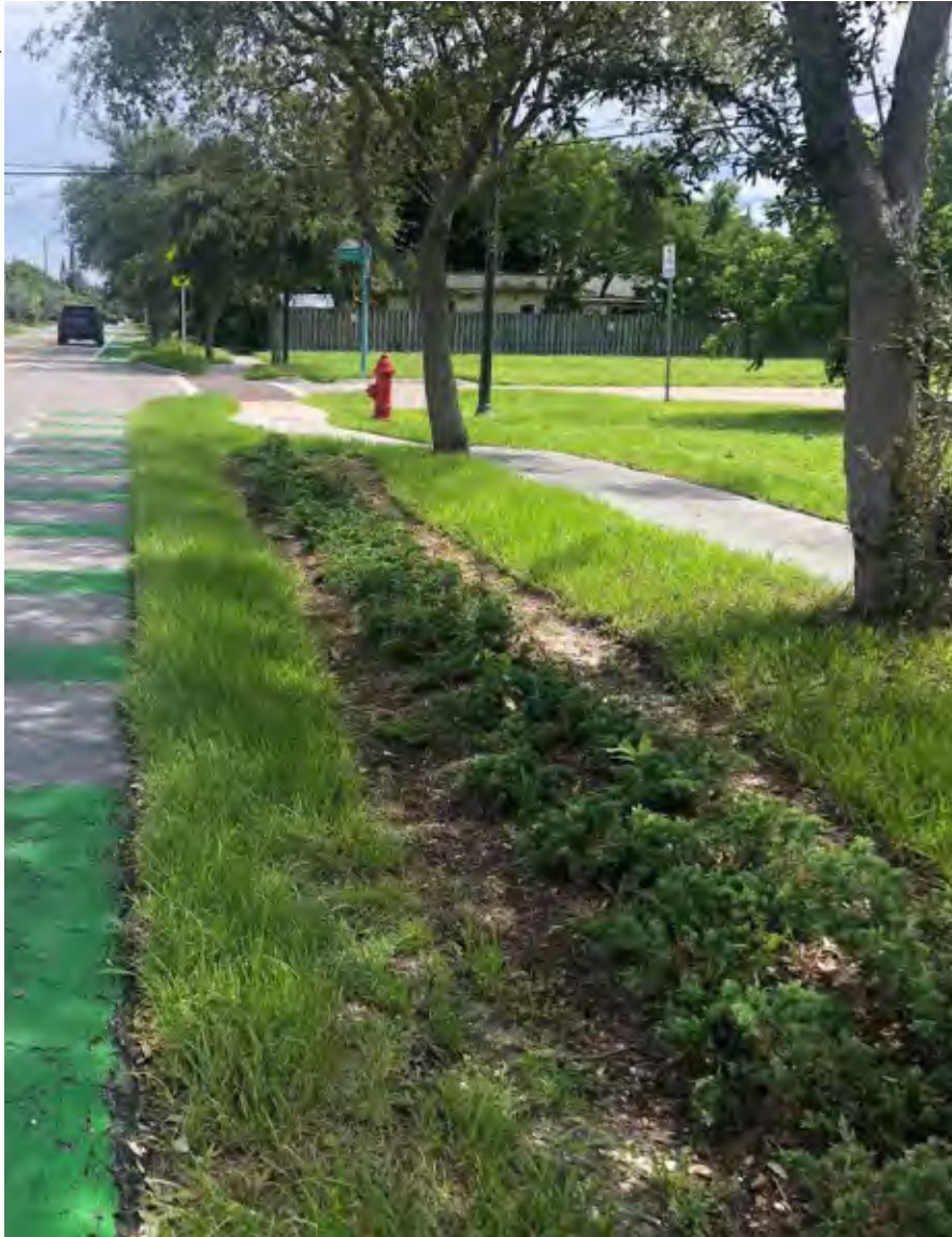
Curbless bioretention with a VFS that treats sheet flow in Fort Lauderdale, FL.
