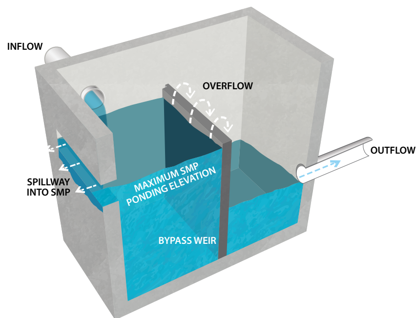
A schematic of a flow splitter for a stormwater management practice (SMP).
