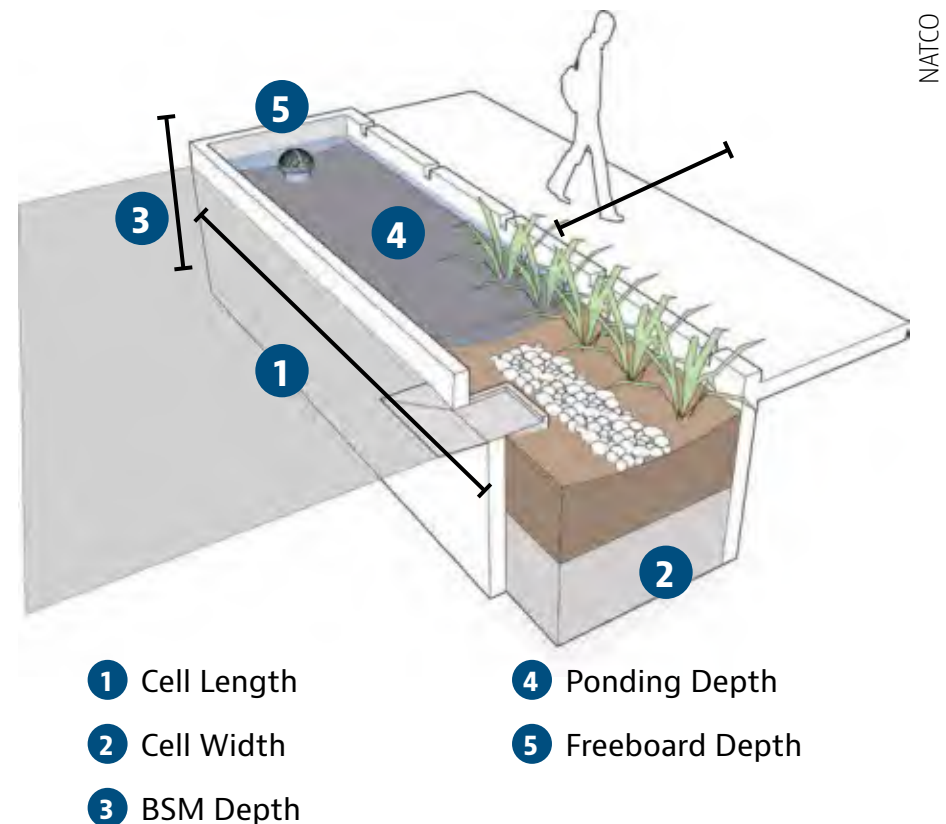
Bioretention planter design schematic.
