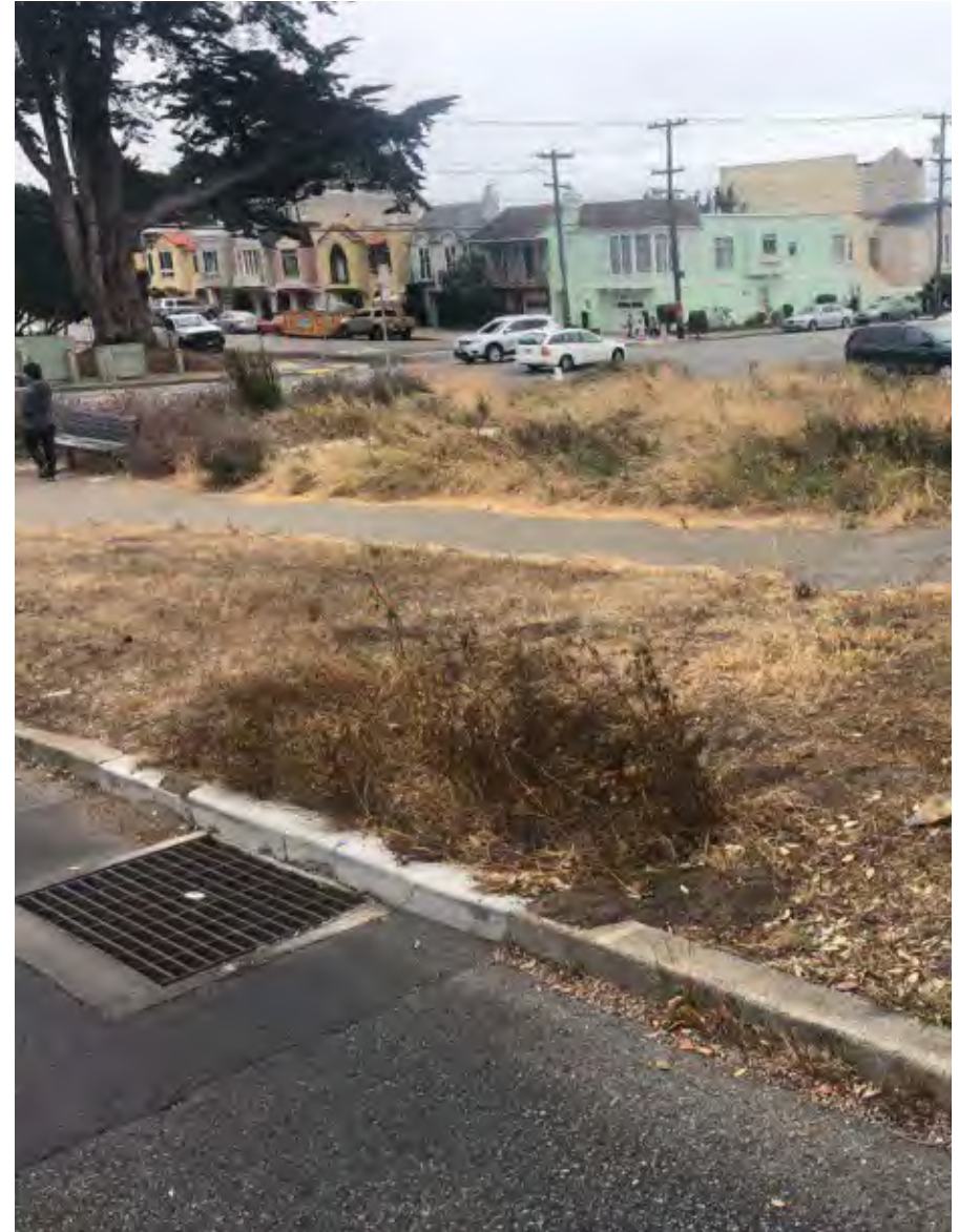
A pipe conveys runoff from a depressed drain to a bioretention facility in San Francisco, CA.
